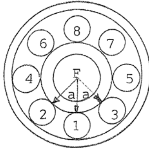
Exaggerated View Showing Effect of Radial Load on Ball Force Distribution
